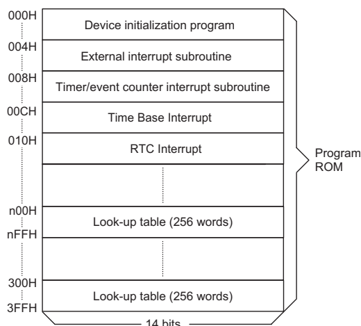
Program Memory
